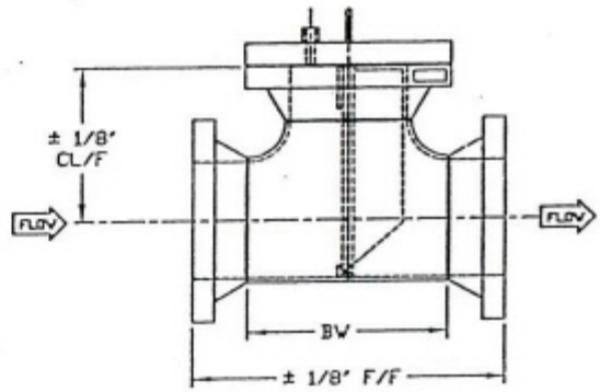
Tee Straight Flow Strainer
