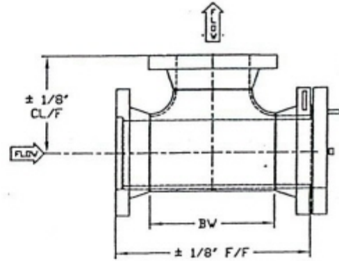
Angle Flow Tee Strainer
