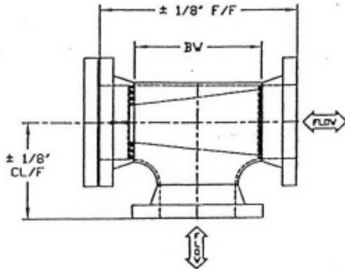
Bi-Directional Angle Flow Tee Strainer
