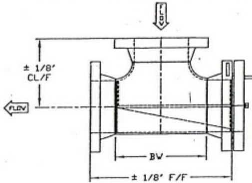
Bi-Directional Angle Flow Tee Strainer
